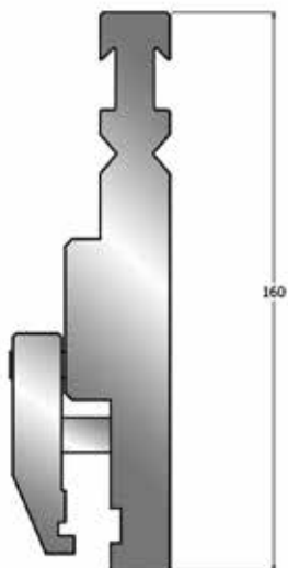
Adaptor RFA-EuroB
